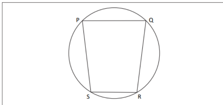
FIGURE 4: Cyclic quadrilateral PQRS.
