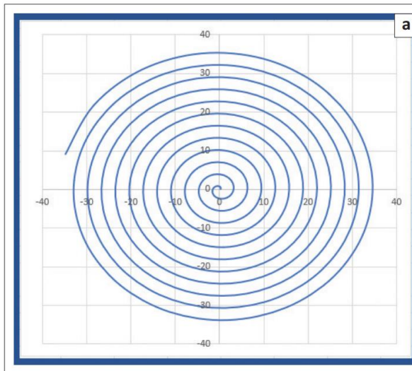
FIGURE 3: Geometrical representation of a spiral.
