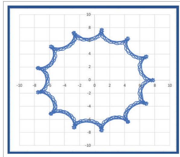
FIGURE 7: Geometrical representation of a concave function.
