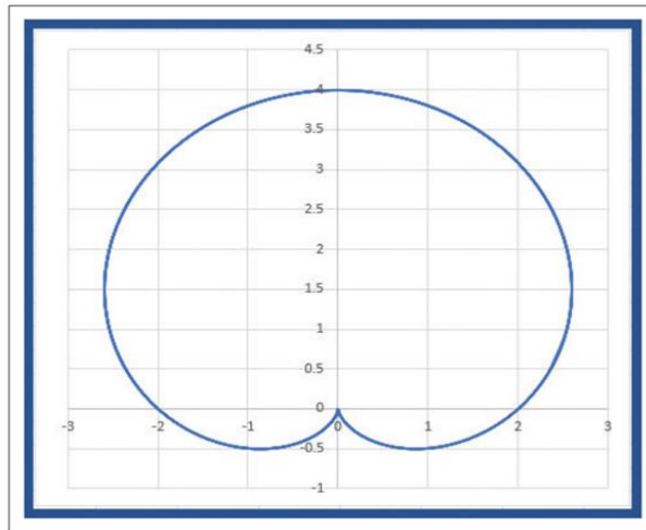
FIGURE 1: Geometrical representation of a cardioid. FIGURE 2: Geometrical representation of a rose.
